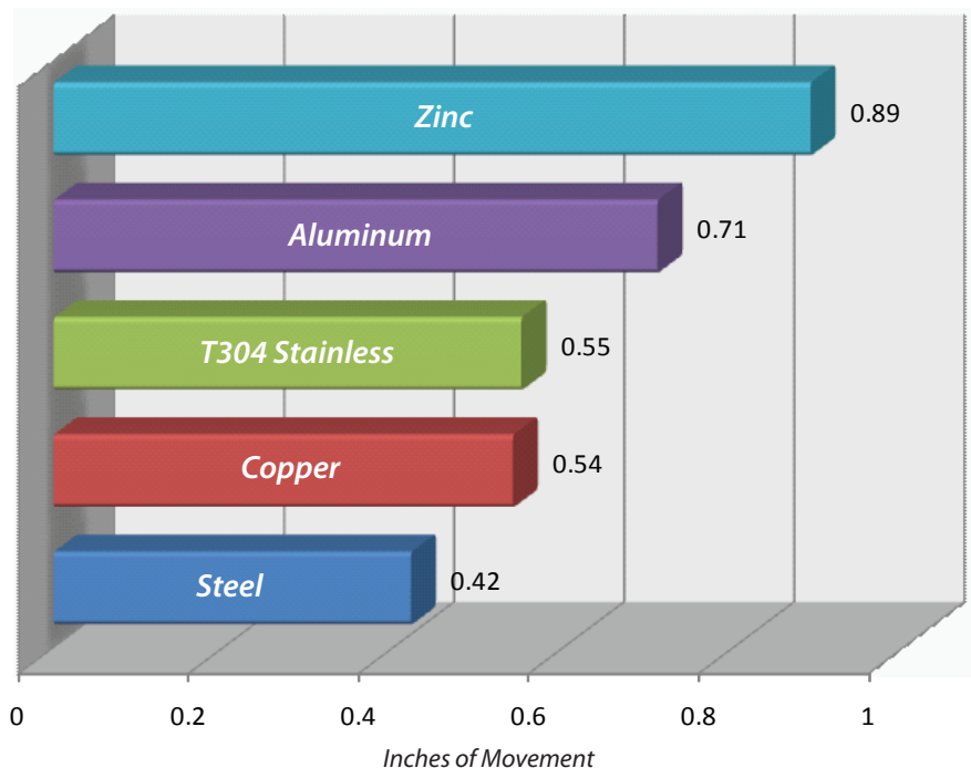
Thermal Movement in 30-foot Lengths at 160 Degree Fahrenheit Temperature Differential
